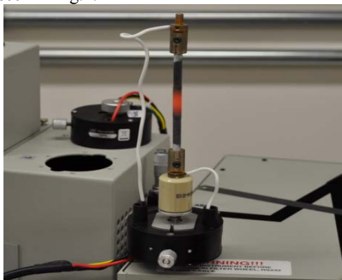
Fig. 4. Silicon Carbide element at 1075K, used as a gray body.
